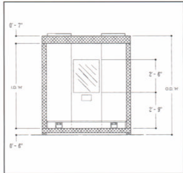
40act Series Typical Elevation
